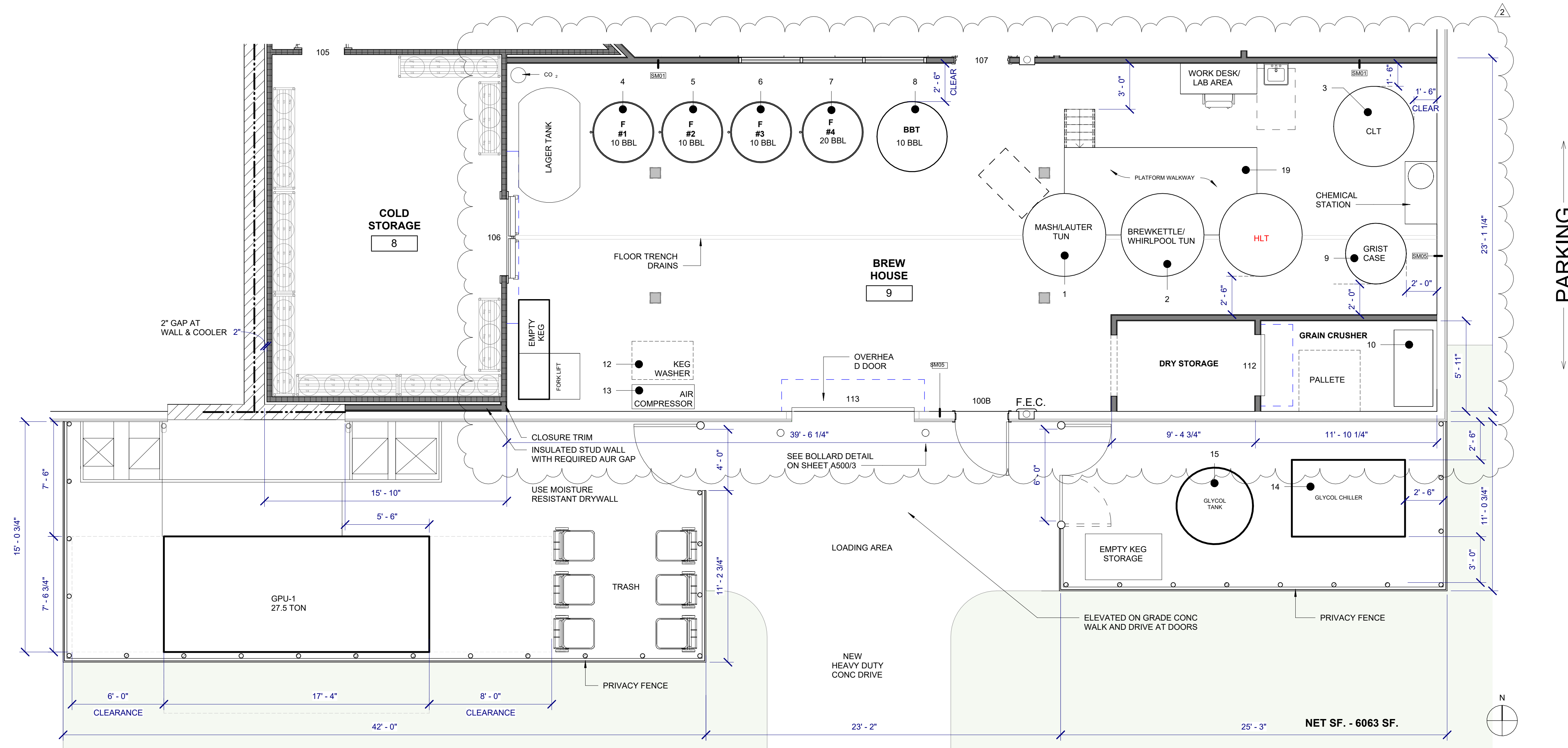
BREWERY FLOOR PLAN - ENLARGED 1/4" = 1'-0" 1
